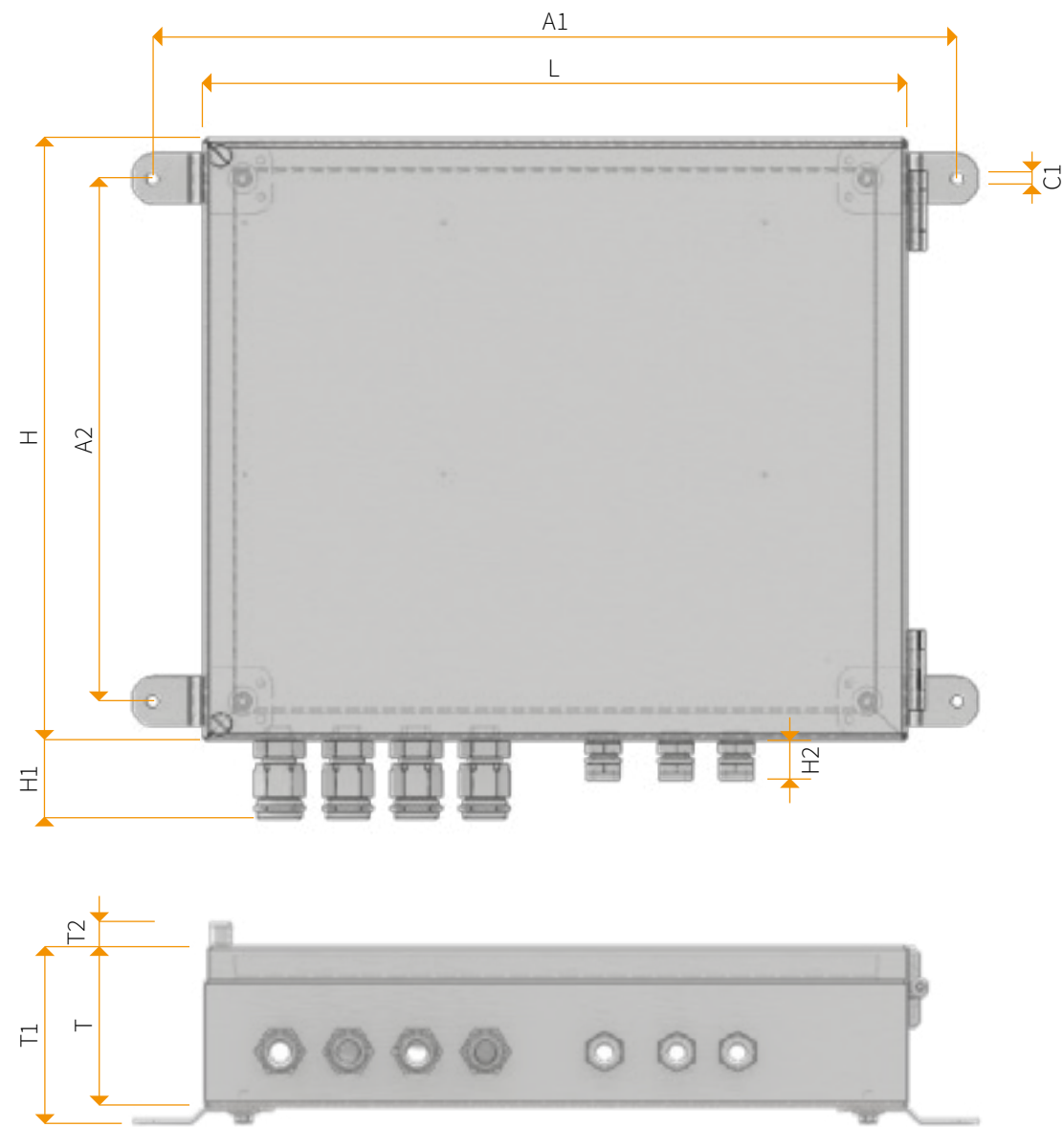
Figure 2: Standard dimensions of the StripKraft Controller (MMV)
