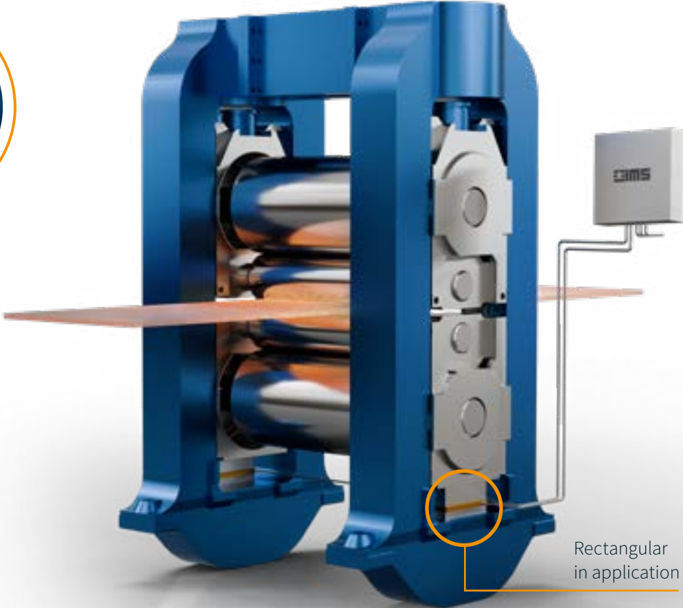
Figure 1: Illustration of a rolling stand equipped with RollKraft Rectangular and RollKraft Controller (MMV) in application
