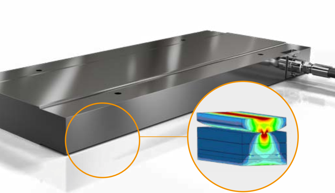
Figure 2: Simulation of force distribution RollKraft Rectangular in application
